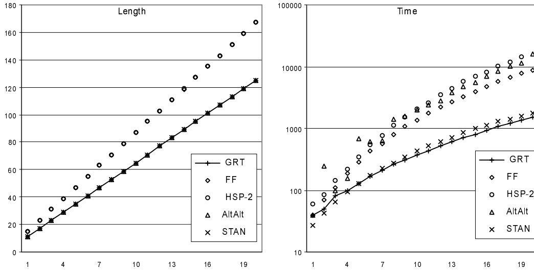
Figure 20: Solution length and time (msecs) in the gripper domain.
