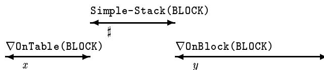
Figure 16: Temporal dependencies in the definition of the Simple-Stack action.
