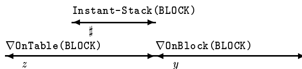
Figure 17: Temporal dependencies in the definition of the Instant-Stack action.
