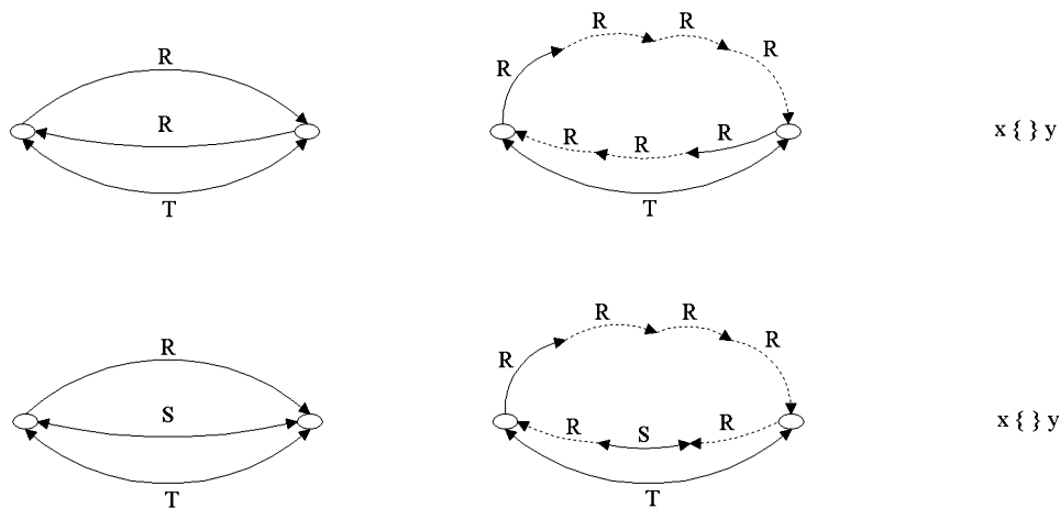
Figure 5: Contradictions in G_{99} : \{\} indicates \perp and R, S, T respectively \{CG, CGPP\} , \{CG, CNO\} and \{CGPP, CGPP^{-1}, CNO\} .
