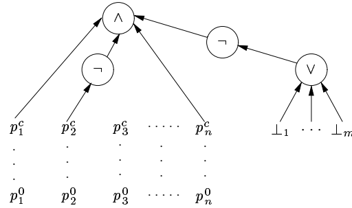
Figure 5: Circuit structure and goal testing for a c -step \mathcal{S}_{\mathcal{L}\mathcal{C}} plan
