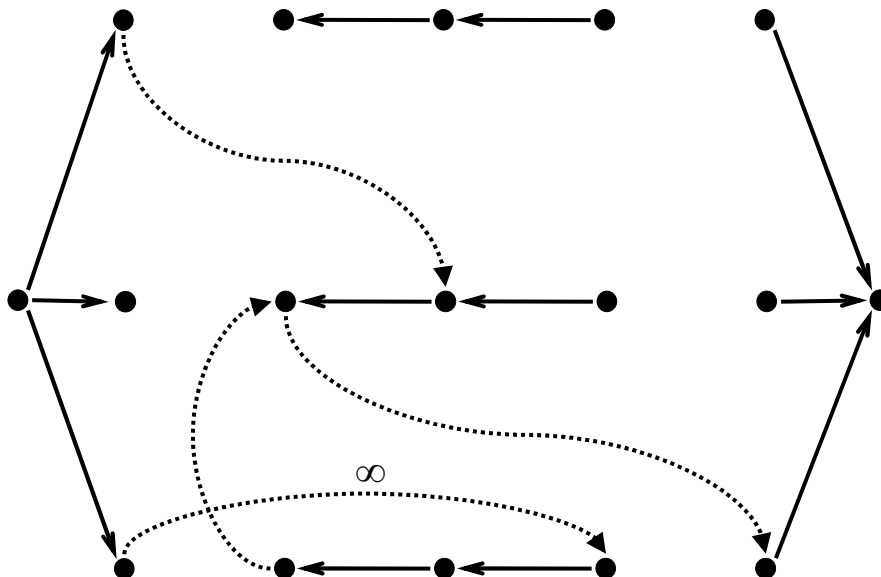
Figure 2: The graph G_{\mathcal{P}} associated with the instance \mathcal{P} defined in Example 3.3. (Note that solid arrows indicate edges with infinite weight.)
