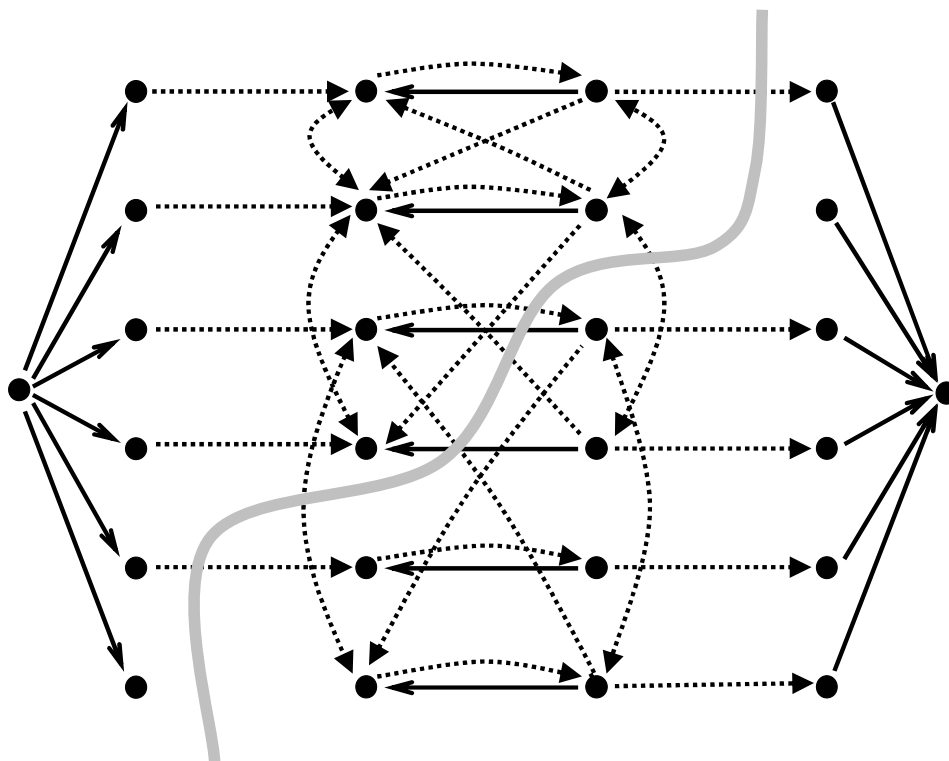
Figure 6: The graph G_{\mathcal{P}} associated with the instance \mathcal{P} defined in Example 5.6.
