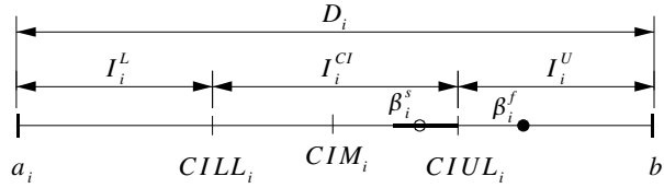
Figure 2: An example of confidence interval based crossover
