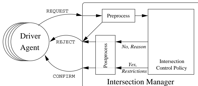
Figure 1: One of the driver agents attempts to make a reservation. The intersection manager responds based on the decision of an intersection control policy.
