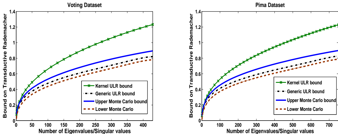
Figure 1: A comparison of transductive Rademacher bounds.
