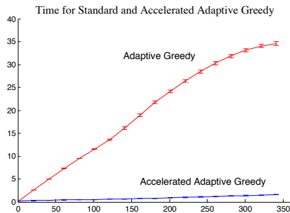
(b) Traffic Data: Execution time (sec) for the naive vs accelerated implementations of adaptive greedy vs. the budget k on number of sensors selected, when p_{fail}(v) = 0.5 for all v , plotted with standard errors.
