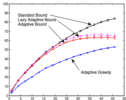
(e) Temperature Data: Rewards & bounds on the optimal value when p_{fail}(v) = 0.5 for all v vs. the budget k on number of sensors selected, plotted with standard errors.
