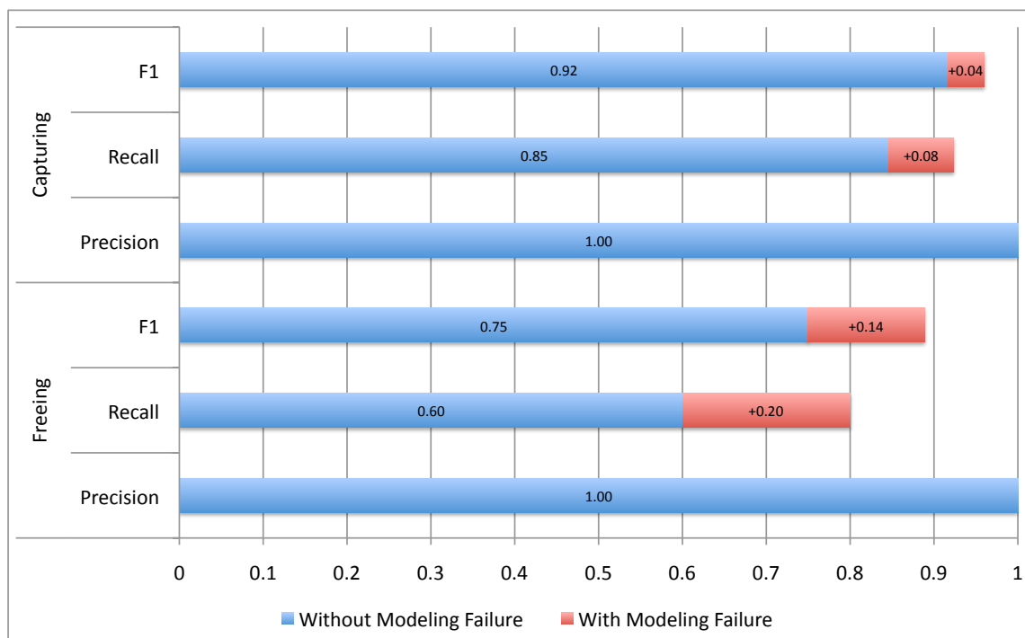
Figure 11: Considering unsuccessfully attempted activities strictly improves performance on standard activity recognition. Blue bars show scores obtained with the unified Markov logic model that considers only successful activities ( \mathcal{M}_S ). The red bars indicate the additive improvement provided by the augmented model that considers both successful and failed activities ( \mathcal{M}_{S+F} , the output of Algorithm 1). Each model labels its target activities jointly, we separate capturing and freeing in the plot for clarity. Precision has value of 1 for both models. F1 scores obtained when explicitly modeling failed attempts are not statistically different from F1 scores obtained without modeling attempts at a high confidence level (p-value of 0.20). However, these results still show the importance of reasoning about people’s attempts when recognizing their activities; see text for details.
