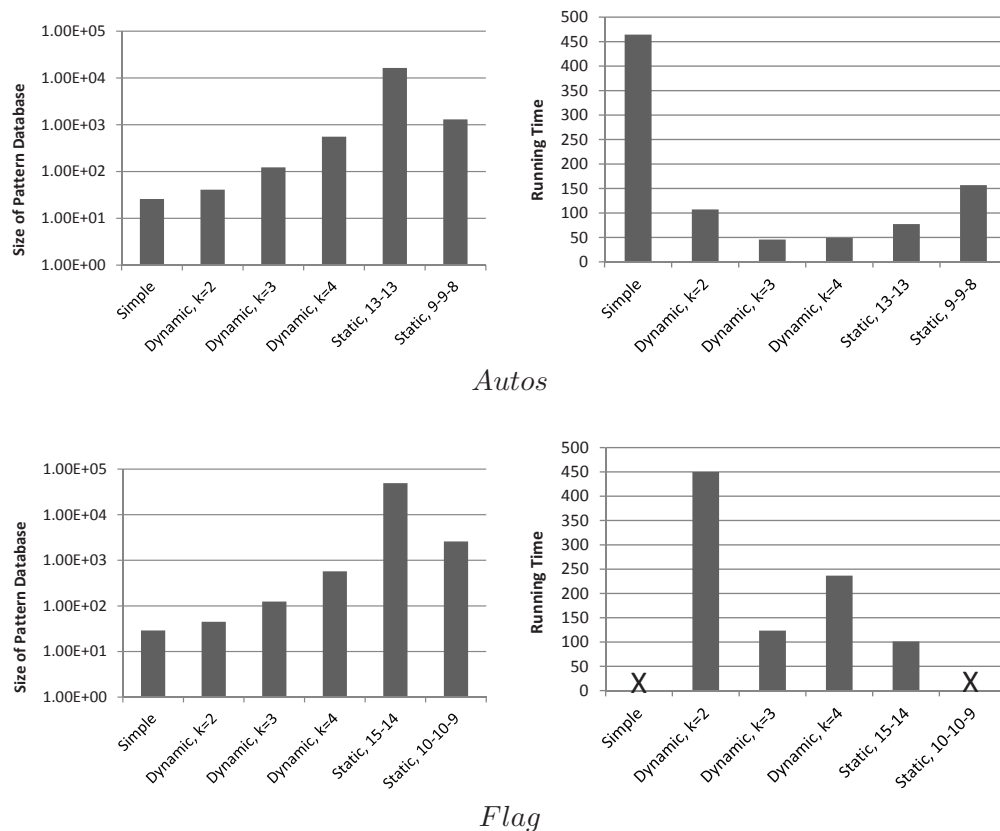
Figure 6: A comparison of A* enhanced with different heuristics ( h_{simple} , h_{dynamic} with k = 2, 3, and 4, and h_{static} with groupings 9-9-8 and 13-13 for the Autos dataset and groupings 10-10-9 and 15-14 for the Flag dataset). “Size of Pattern Database” means the number of patterns stored. “Running Time” means the search time (in seconds) using the indicated pattern database strategy. An “X” means out of memory.
