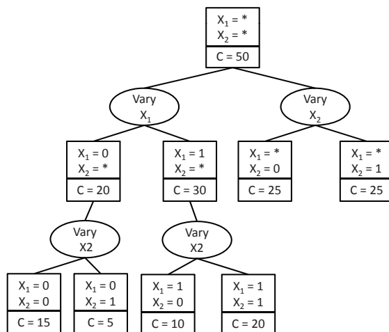
Figure 3: An AD-tree.
