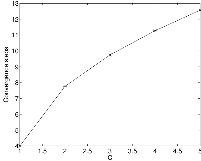
Figure 10: Market convention: Expected number of convergence steps given K = 2 , \delta = 0.9 , \gamma = 1.0 and varying number of resources C and agents N = 2 \cdot C .
