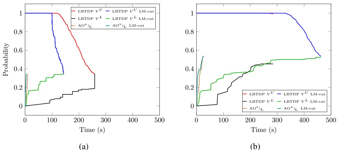
Figure 7: Acyclic planning. Anytime behavior in \text{LRTDP}_{|\text{L}}_{\text{U}} ( V^U and V^L ) and \text{AO}^*_{|\text{L}} ( V^L only), as a function of runtime. Elevators instance 11, without pruning and with LM-cut pruning, for constrainedness level C = 1.4 (a) respectively C = 1.8 (b). Default node selection.
