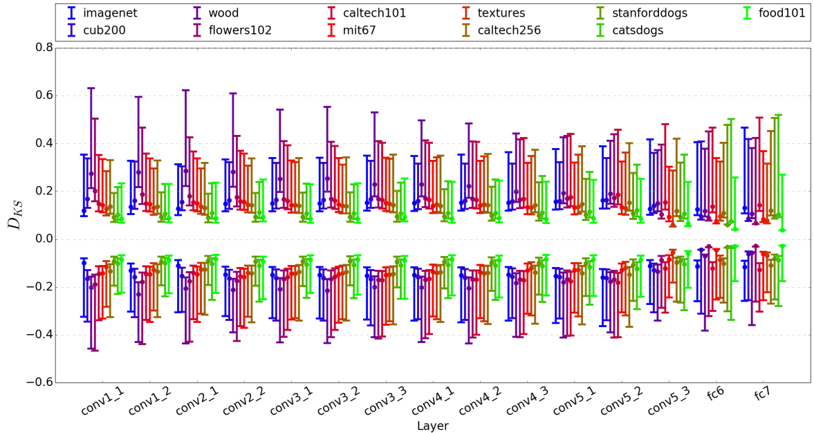
Figure 5: Inner/outer class D_{KS} distribution per layer for 11 different datasets on the embedding. Since the distribution of D_{KS}^+ and D_{KS}^- is similar to a log-normal distribution we represent it by the mode at the central point and two error bars enclosing 68% of accumulated probability on each side (equivalent to \mu \pm \sigma for normal distribution).
