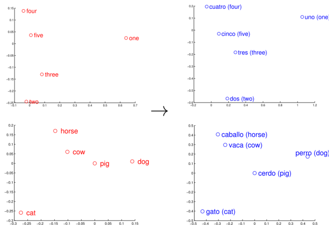
Figure 3: Similar geometric relations between numbers and animals in English and Spanish (Mikolov et al., 2013b). Words embeddings are projected to two dimensions using PCA and were manually rotated to emphasize similarities.
