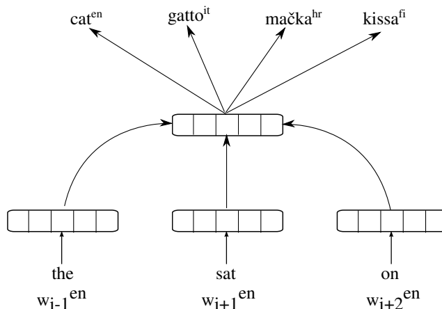
Figure 5: Illustration of the joint multilingual model of Duong et al. (2017) based on the modified CBOW objective; instead of predicting only the English word given the English context, the model also tries to predict its translations in all the remaining languages (i.e., in languages for which the translations exist in any of the input bilingual lexicons).
