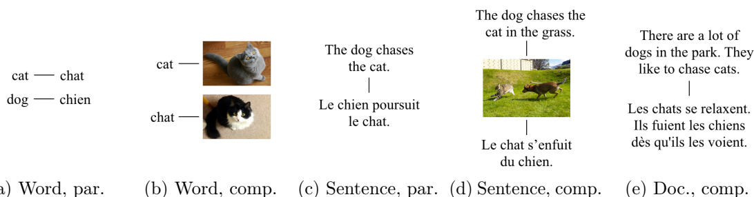
Figure 2: Examples for the nature and type of alignment of data sources. Par.: parallel. Comp.: comparable. Doc.: document. From left to right, word-level parallel alignment in the form of a bilingual lexicon (2a), word-level comparable alignment using images obtained with Google search queries (2b), sentence-level parallel alignment with translations (2c), sentence-level comparable alignment using translations of several image captions (2d), and document-level comparable alignment using similar documents (2e).
