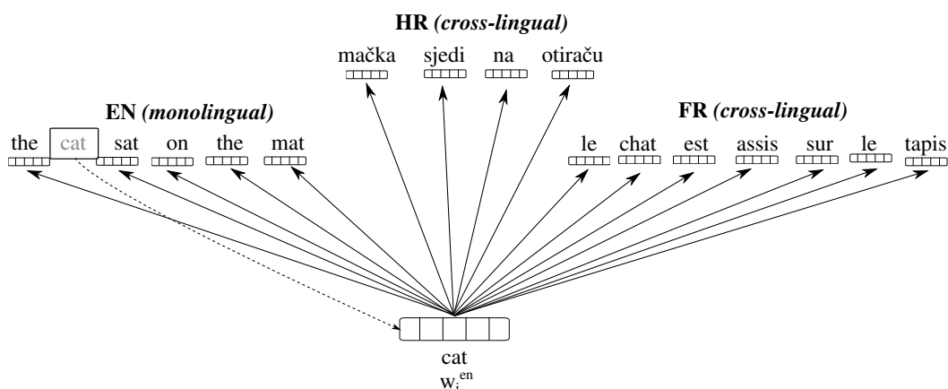
Figure 6: A multilingual extension of the sentence-level TransGram model of Coulmance et al. (2015). Since the model bypasses the word alignment step in its SGNS-style objective, for each center word (e.g., the EN word cat in this example) the model predicts all words in each sentence (from all other languages) which is aligned to the current sentence (e.g., the EN sentence the cat sat on the mat ).
