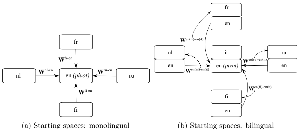
Figure 4: Learning shared multilingual embedding spaces via linear mapping. (a) Starting from monolingual spaces in L languages, one linearly maps L - 1 into one chosen pivot monolingual space (typically English); (b) Starting from bilingual spaces sharing a language (typically English), one learns mappings from all other English subspaces into one chosen pivot English subspace and then applies the mapping to all other subspaces.
