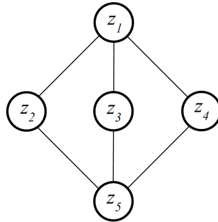
Figure 16: A graph with girth 4.
