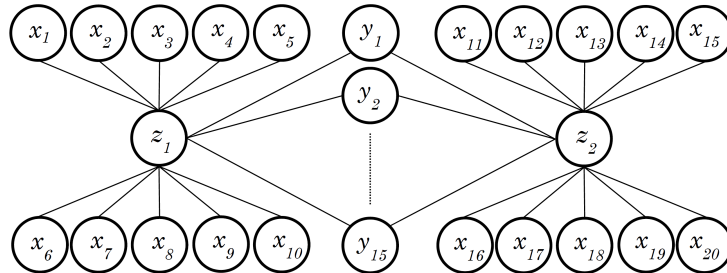
Figure 1: A SDG not converging to a Nash equilibrium.
