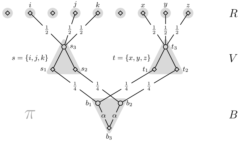
Figure 7: Schematic of the reduction for the verification problem of popular partitions on bipartite FHGs. The bipartition is indicated by the shapes of the agents. The partition \pi under consideration is marked in gray.
