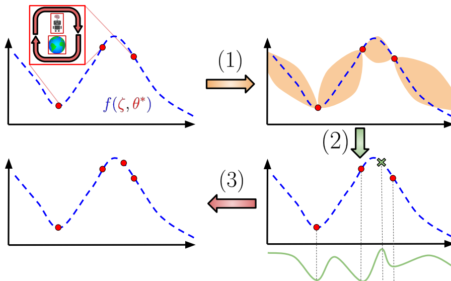
Figure 4: Bayesian Optimization, which consists of 3 main steps. (1): A regressor (commonly a Gaussian Process) is used to construct uncertainty estimates on the blackbox function f(\cdot) given previous evaluation data. (2): An acquisition function is constructed from the regressor, which represents the explore-exploit tradeoff on f . (3): The argmax of the acquisition function is used for the next trial.
