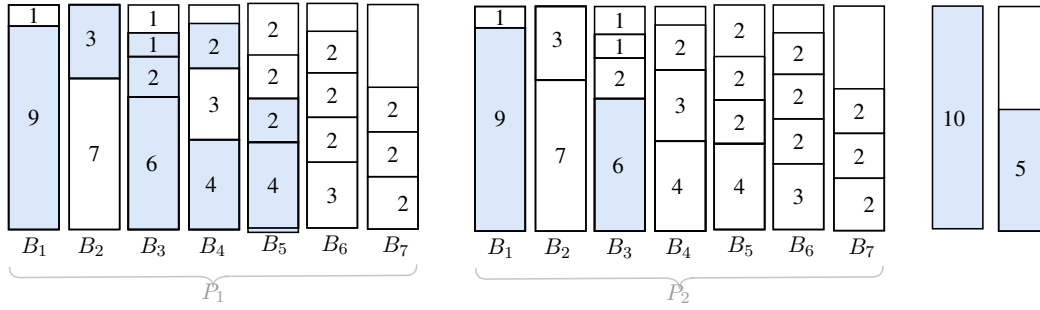
Figure 1: The packing output by PROFILEPACKING on the input sequence \sigma = 2, 3, 1, 4, 10, 2, 9, 4, 6, 9, 2, 6, 5 . The predictions and the corresponding profile are as given in Example 1. The optimal packing of the profile consists of seven bins B_1, \dots, B_7 . When serving \sigma , the algorithm opens two profile groups, denoted by P_1 and P_2 . The profile group P_2 is opened upon serving the second item of size 9, namely the 10th request in the sequence. The placeholders that have received an item are highlighted. Items 10 and 5 are special items and are packed using FIRST-FIT. The total cost for serving \sigma is equal to 9, and there are 7 bins that are only opened virtually, hence they do not contribute to the cost.
